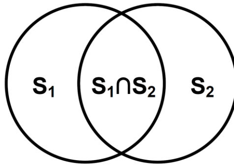
FIG. 6: Overlapping Sets
